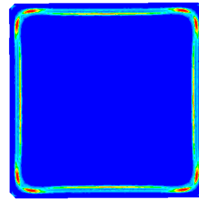
Figure 10. Influence of the casting speed on hot tearing risk, according to the criterion of Yamanaka et al. [18].
