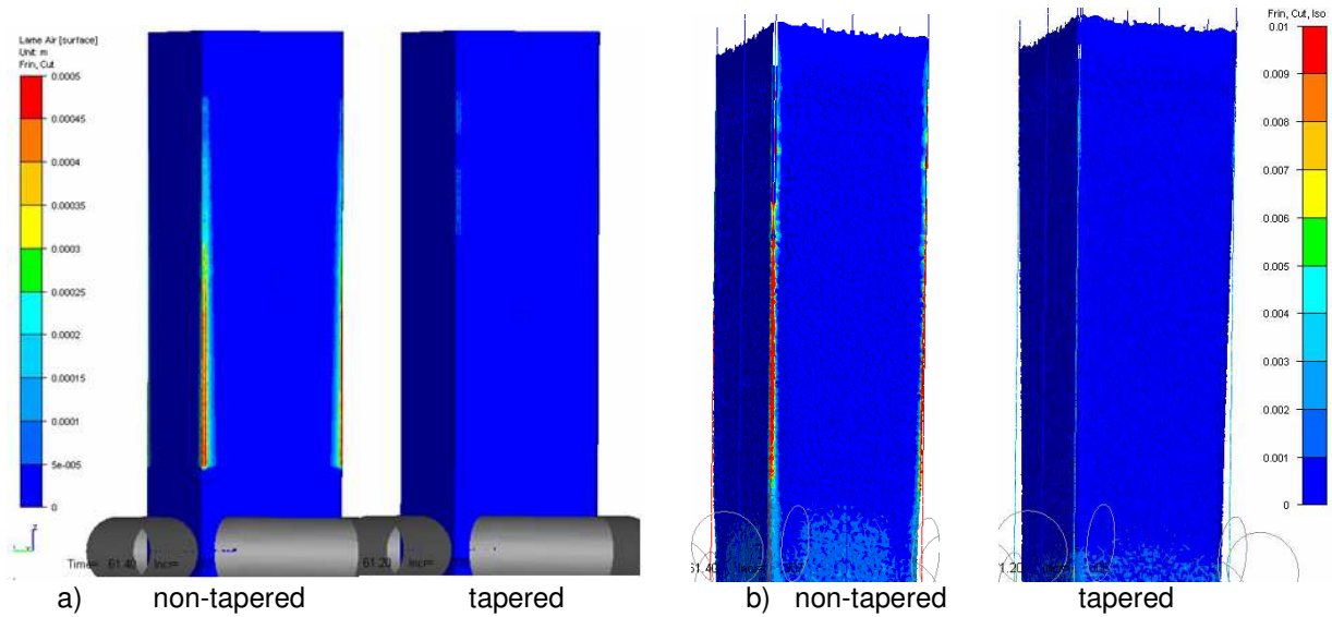
Figure 6. a) Influence of mould tapering on air gap [m] formation.
